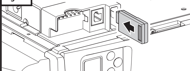
Fig. 42 Modular Antenna Installation or Replacement
